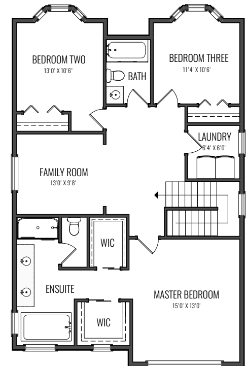
UPPER LEVEL
